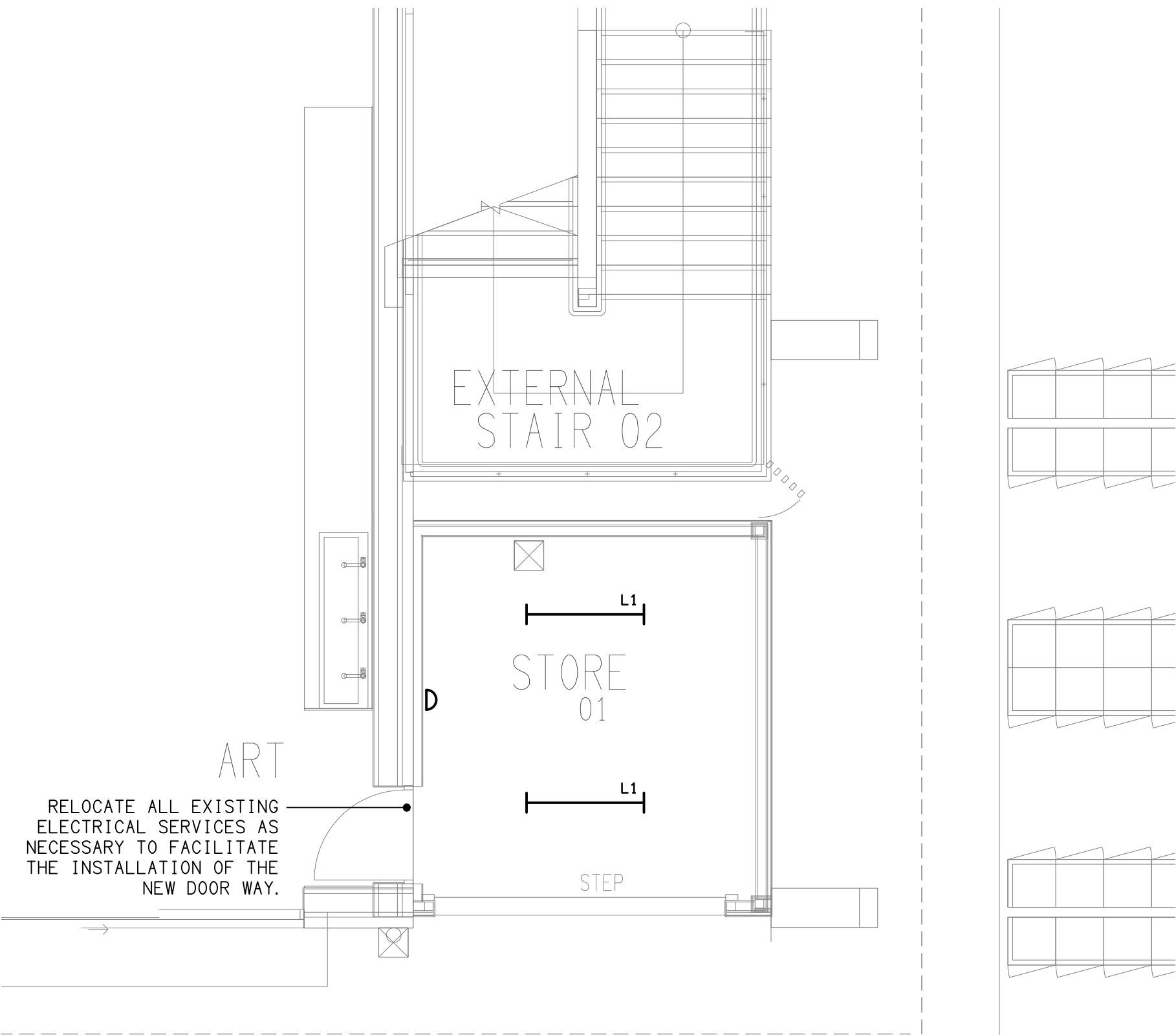
GROUND LEVEL STORE ROOM 1 PLAN SCALE 1: 50
