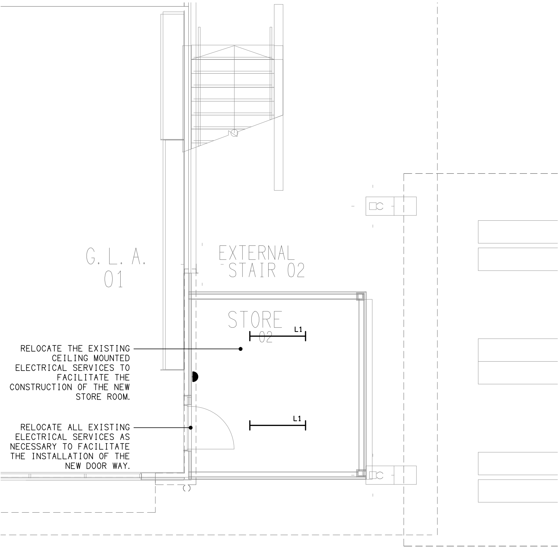
LEVEL 1 STORE ROOM 2 PLAN SCALE 1: 50
